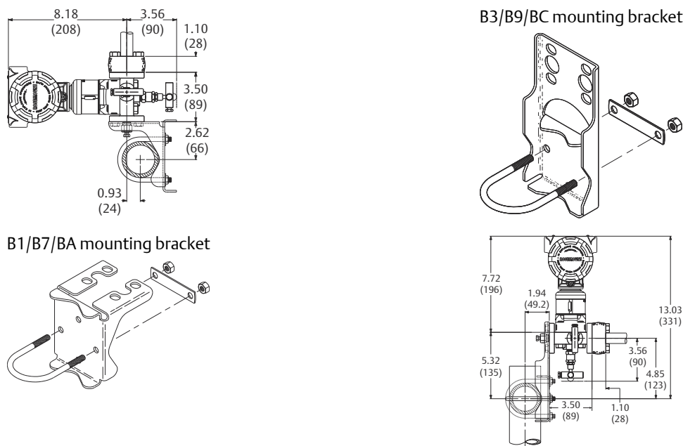
Figure 42: Traditional Manifold with Optional Brackets for 2-in. (50.8 mm) Pipe Mounting
