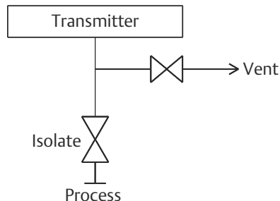
Figure 3: Rosemount 304 Manifold
