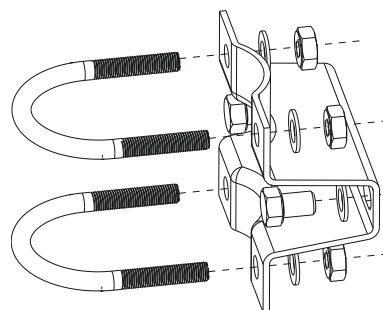
Figure 44: Coplanar Manifold with Optional Bracket for 2-in. (50.8 mm) Pipe Mounting
