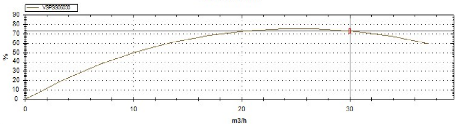
Q-Efficiency Curve
