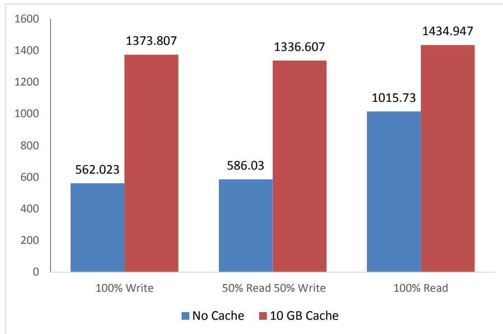
Figure 8.1 Total achieved IOPS for RS3614xs+ (higher is better)
