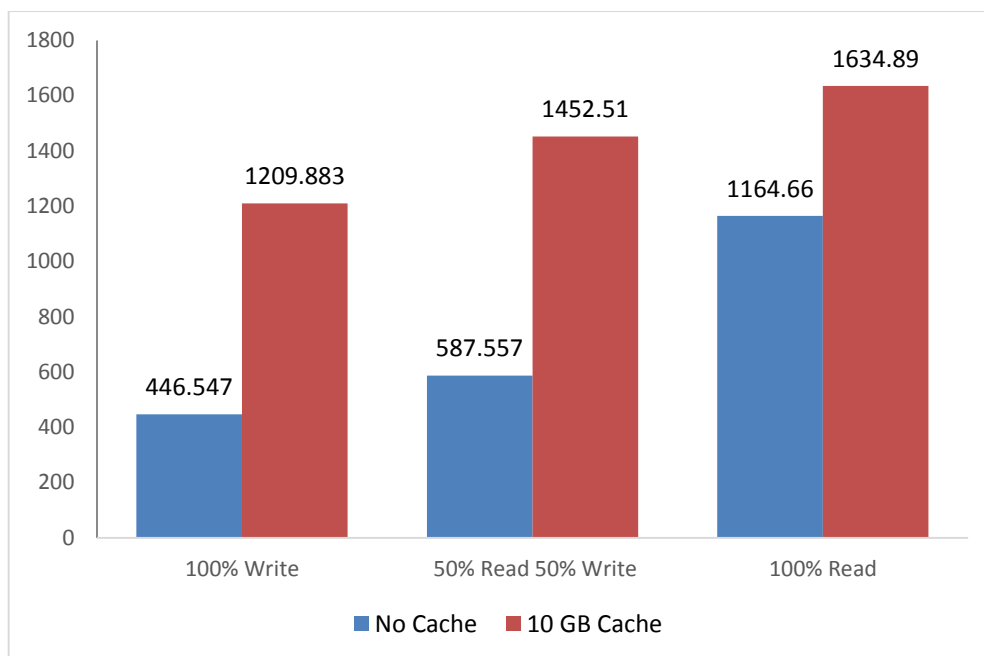
Figure 8.2 Total achieved IOPS for RS2414+ (higher is better)
