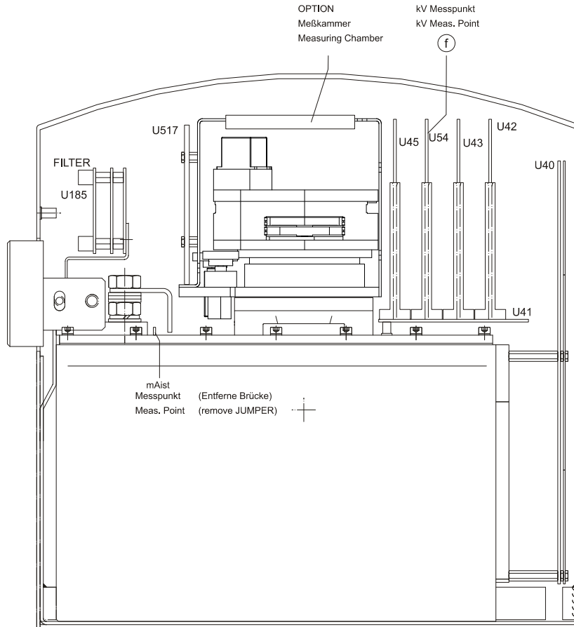
Fig. 8-1 Generator assembly
