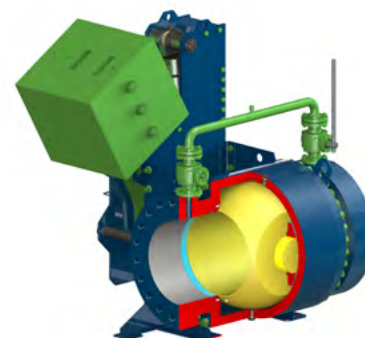
Fig. 9 Ball valve operated with hydro cylinder and counterweight
