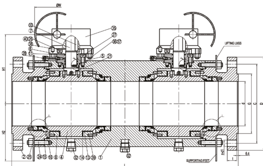
Fig. 7 Twin ball valve
