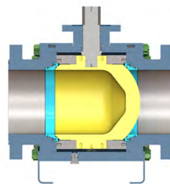
Fig. 8 Pigging ball valve
