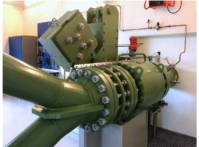
Ball valve at the Norwegian Liarelva hydroelectric power plant
