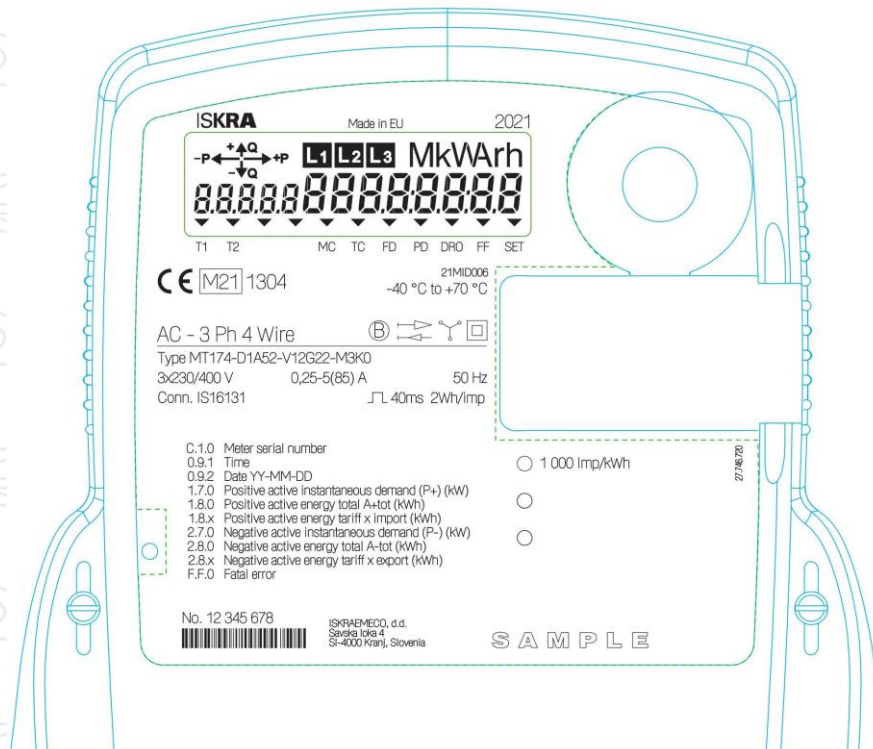
Figure 2: Example of front plate for MT174-D1 meter
