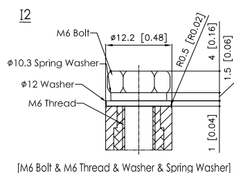
Detail A Drawing(4:1)
