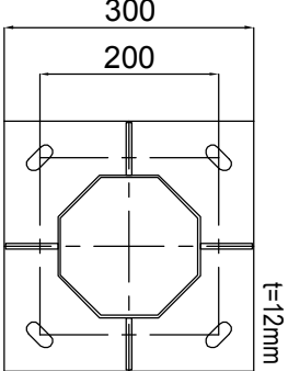
BASE PLATE
