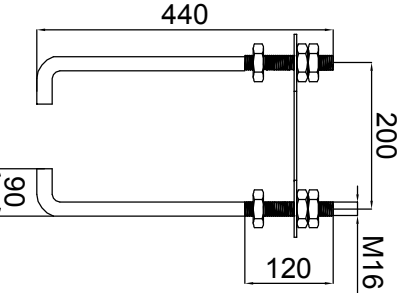
ANCHOR BOLT
