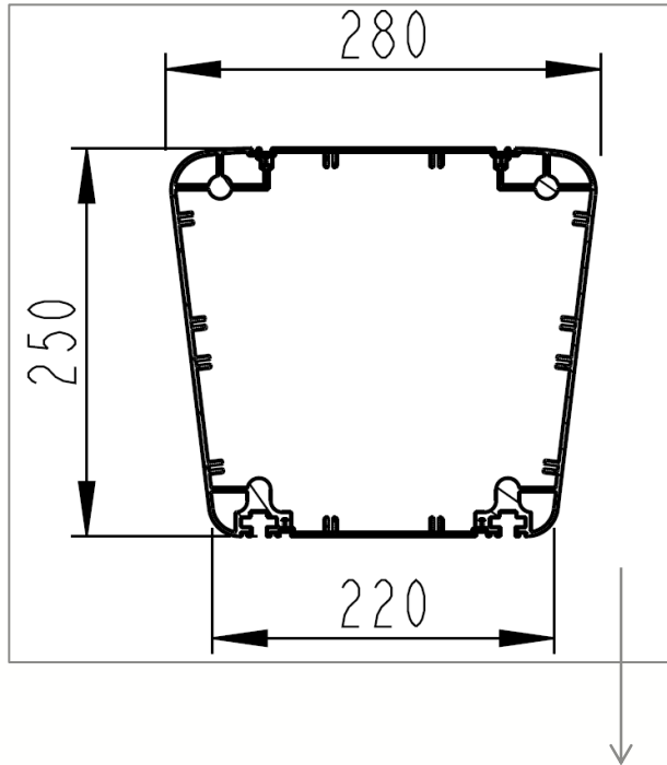
Column profile of Hyport B30
