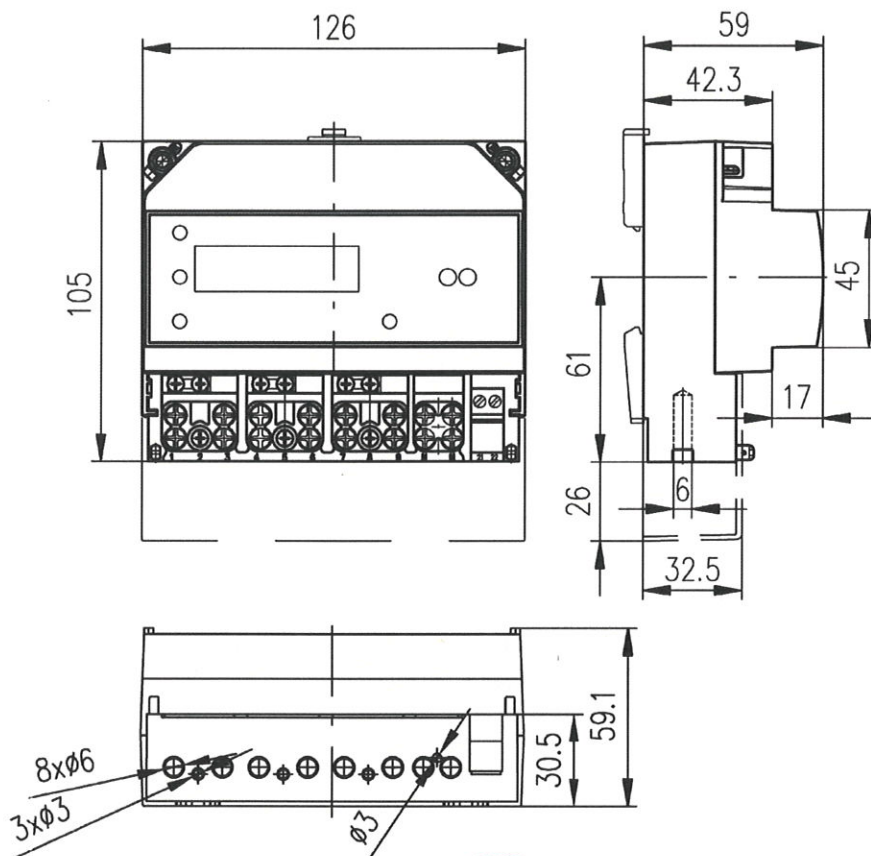
Fig. 2d: View and main dimensions of the electricity meter Applied Meters B2C-FS4TC14 with DIN 35 rail
