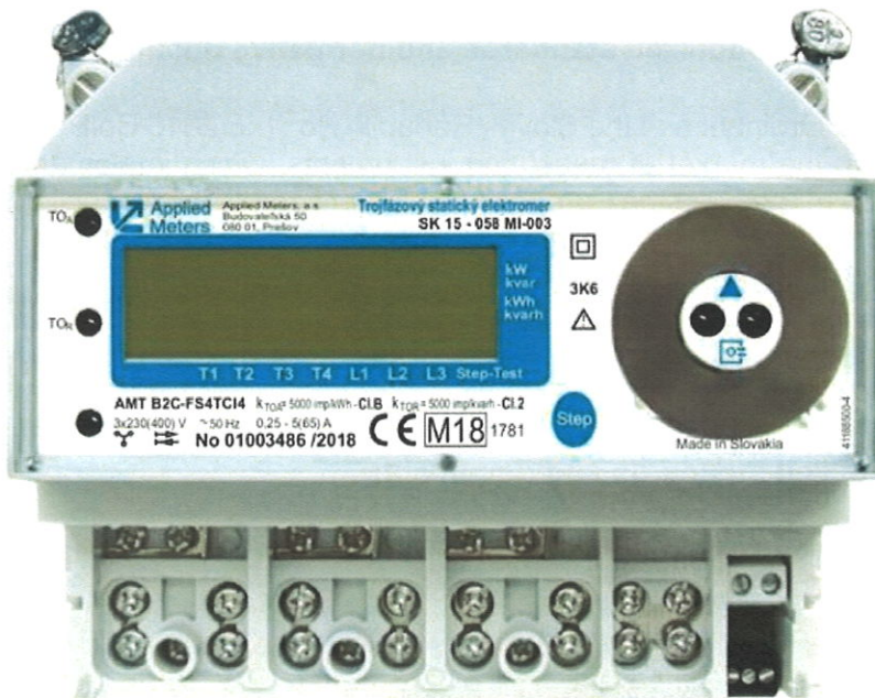
Fig. 1b: Electricity meter Applied Meters AMT B2C-FS4TCI4 with DIN 35 rail
