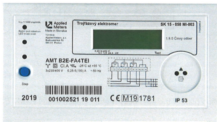
Fig. 3b: Example of marking directly on cover of the electricity meter – Applied Meters AMT B2x-FA4T9I(E) (alternative - by laser printing)
