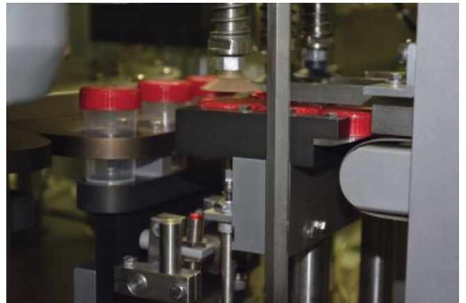
Fig 3.4. Fully automatic Specimen Container production line - Container / cap closure.
