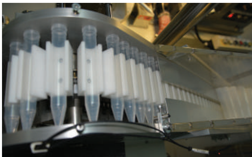
Fig 5.3. Conical Tubes.
