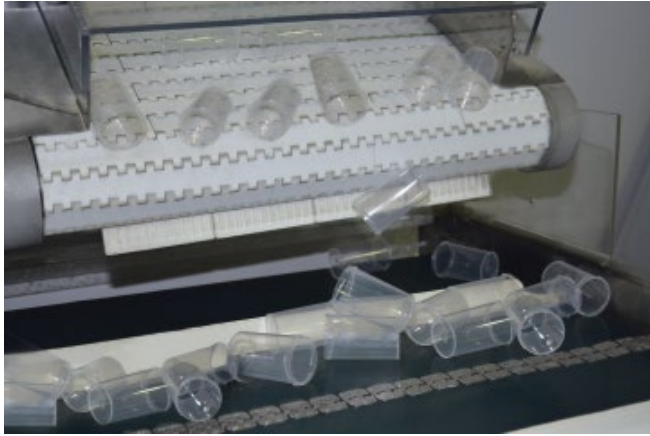
Fig 3.1. Fully automatic Specimen Container production line - Container feeding.
