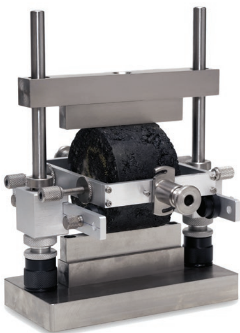
Test set-up for EN 12697-26C, AASHTO TP31, AS 2891.13.1, ASTM D4123 & BS DD213
