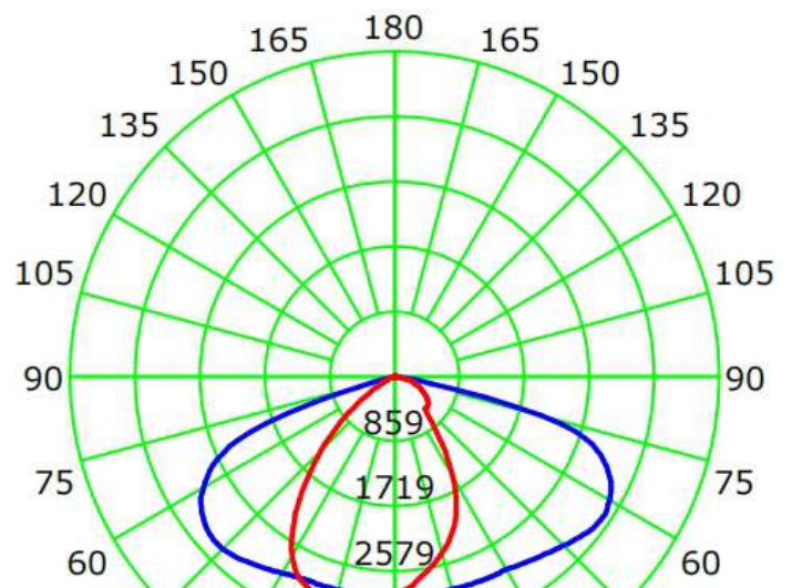
Luminous Intensity Distribution Curve
