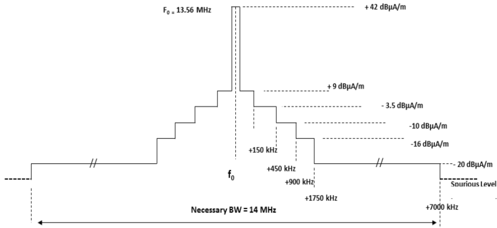
Figure I.3: Spectrum mask limit for wideband RFIDs (incl. NFC application) in the 13,56 MHz range
