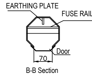
FUSE DETAIL
