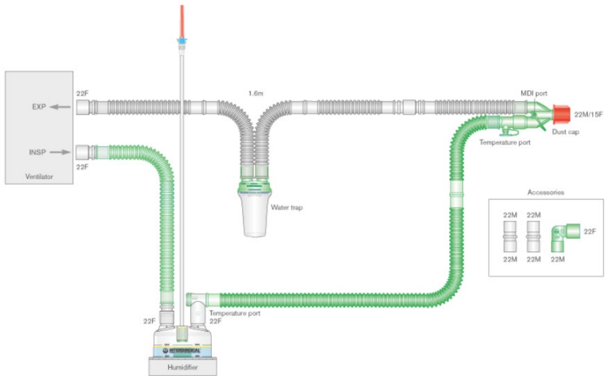
22mm Flextube single heated wire breathing system with water trap, auto-fill chamber and limb. \geq 1.6\text{m}
