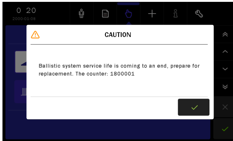
Figure 10.3 The screen with information about approaching necessity of replacing projectile chamber
