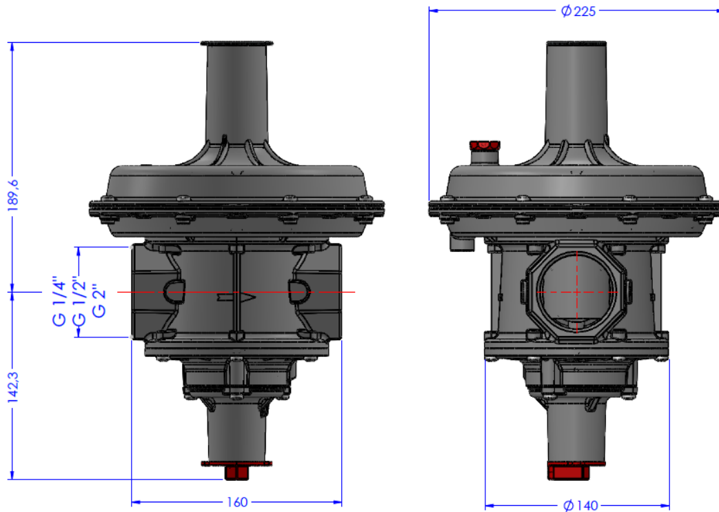
Figure 6: ERG-EH Technical Dimensions
