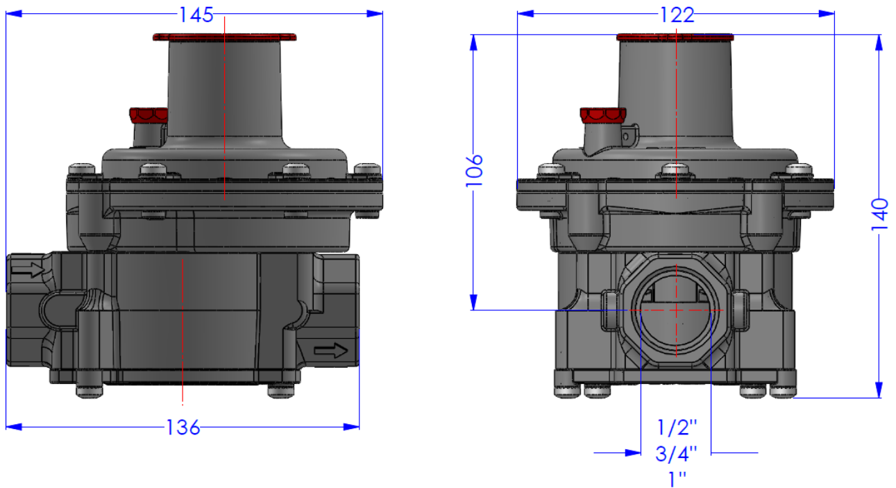
Figure 9: ERG-H Technical Dimensions
