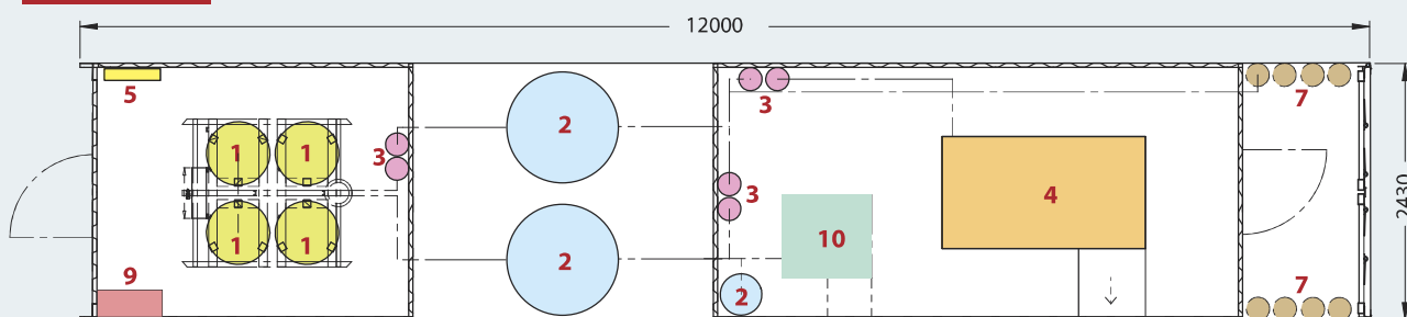
40ft Container
