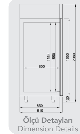
54 adet 36x17x12 Dondurma Kabı Kapasiteli 54 units 36x17x12 Ice Cream Cup Capacity
