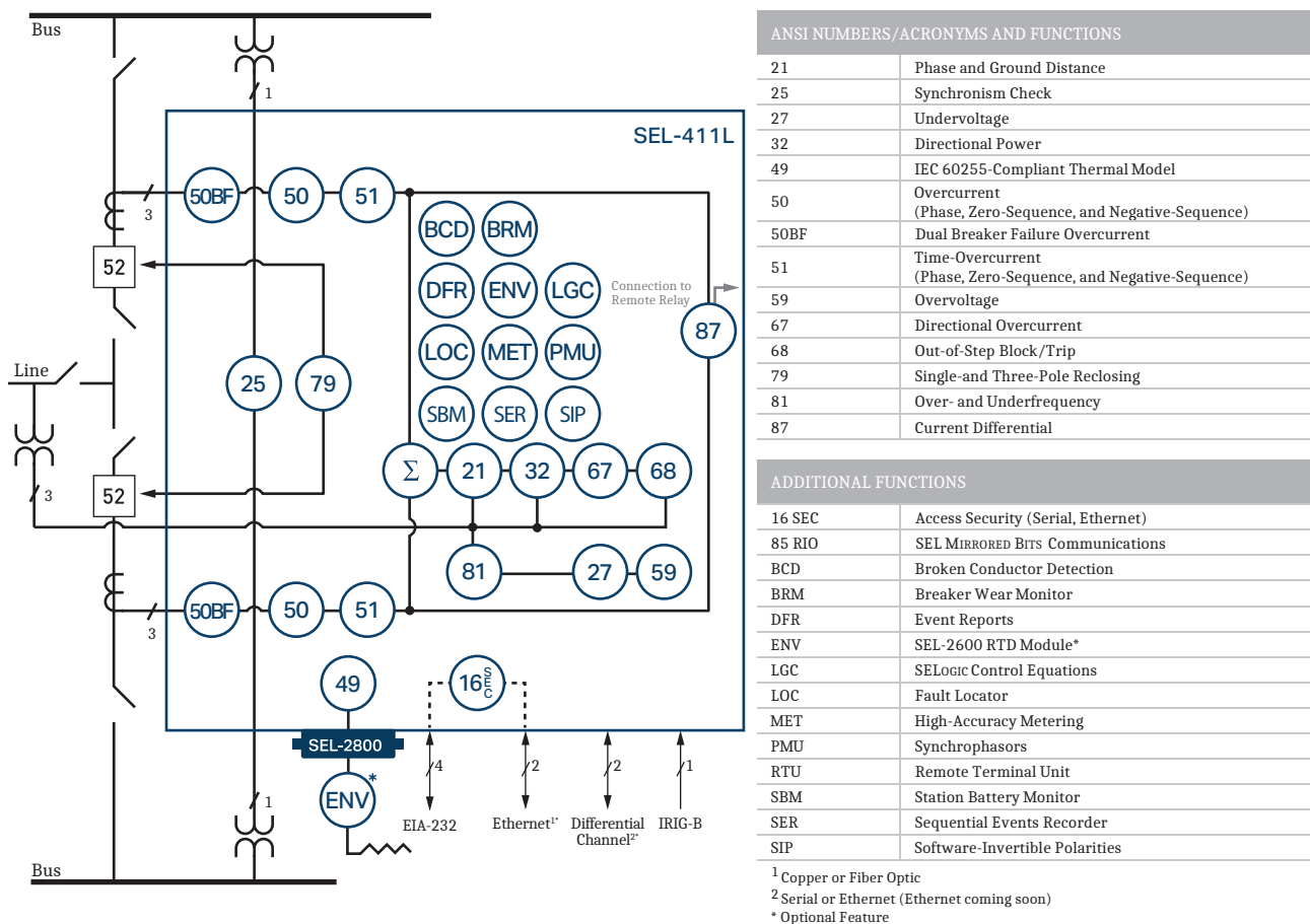
Figure 1 Functional Overview
