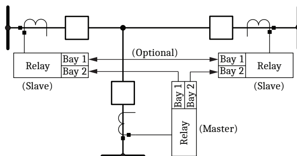
Figure 14 Three-Terminal 3SM Configuration With All Relays as Masters
