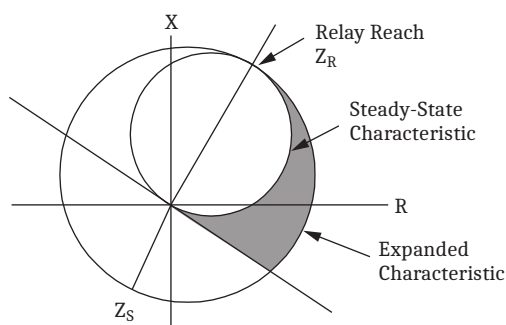
Figure 10 Mho Characteristic
