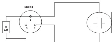
Condenser without internal pull up resistor.
