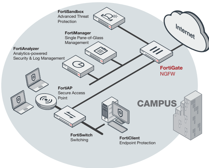
FortiGate 500E/501E deployment in Campus (NGFW)
