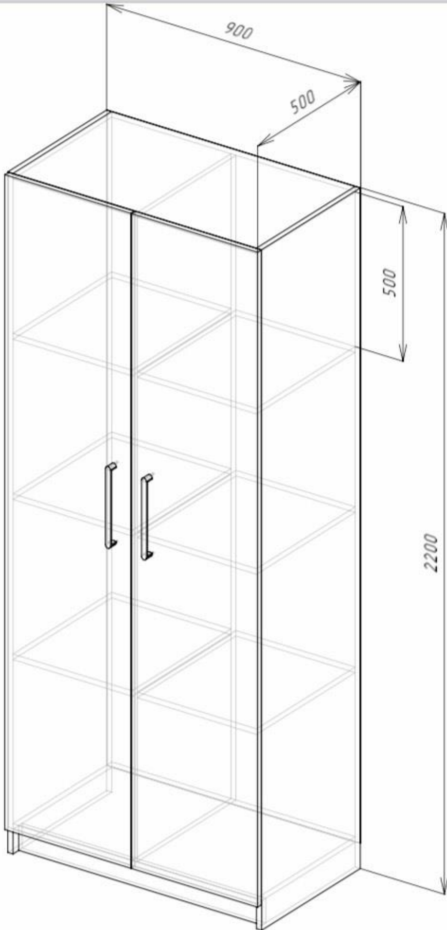
Dulap modular model 2
