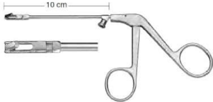
STAMMBERGER BR-7600 Antrum Punch Upside backward cutting
