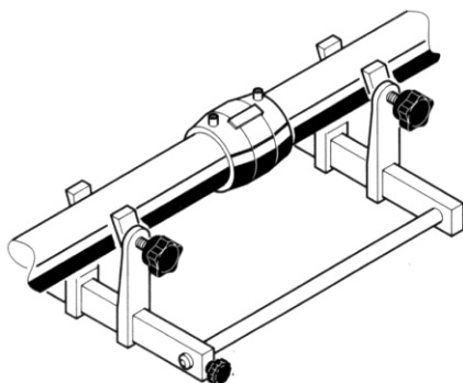
Fig. 2.1 MANȘON ELECTRIC BIFILAR
