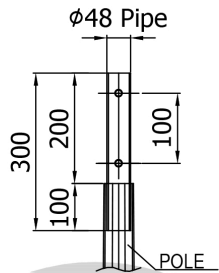
SPIGOT DETAIL
