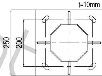
BASE PLATE
