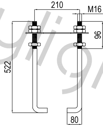
ANCHOR BOLT
