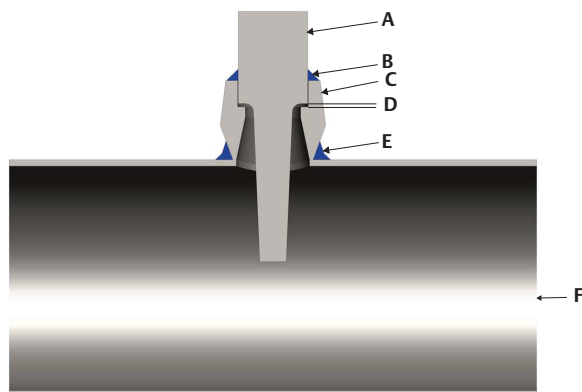
Figure 21. Installation Components
