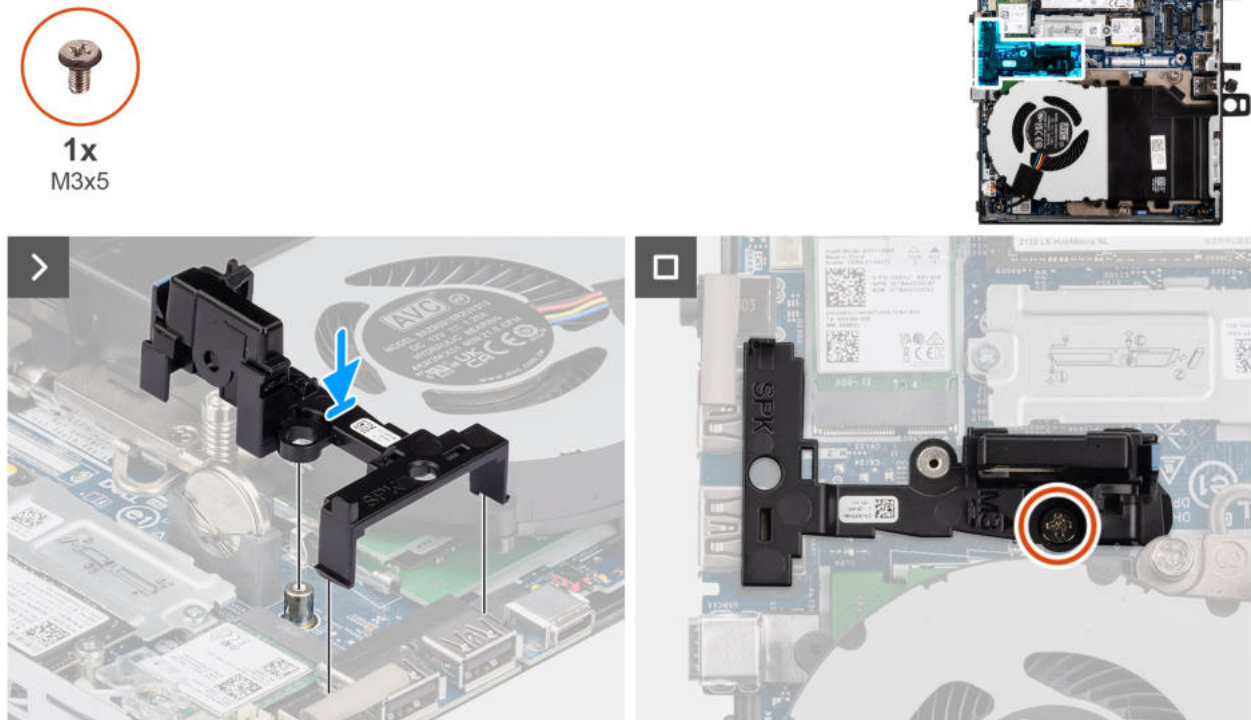
Figure 79. Installing the speaker holder
