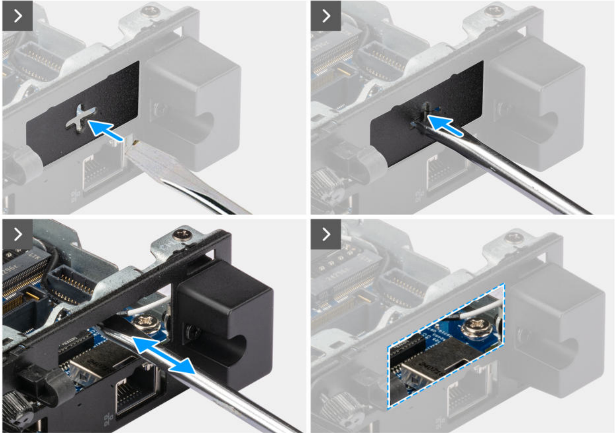
Figure 39. Installing dual USB 3.2 Gen 2 ports module
