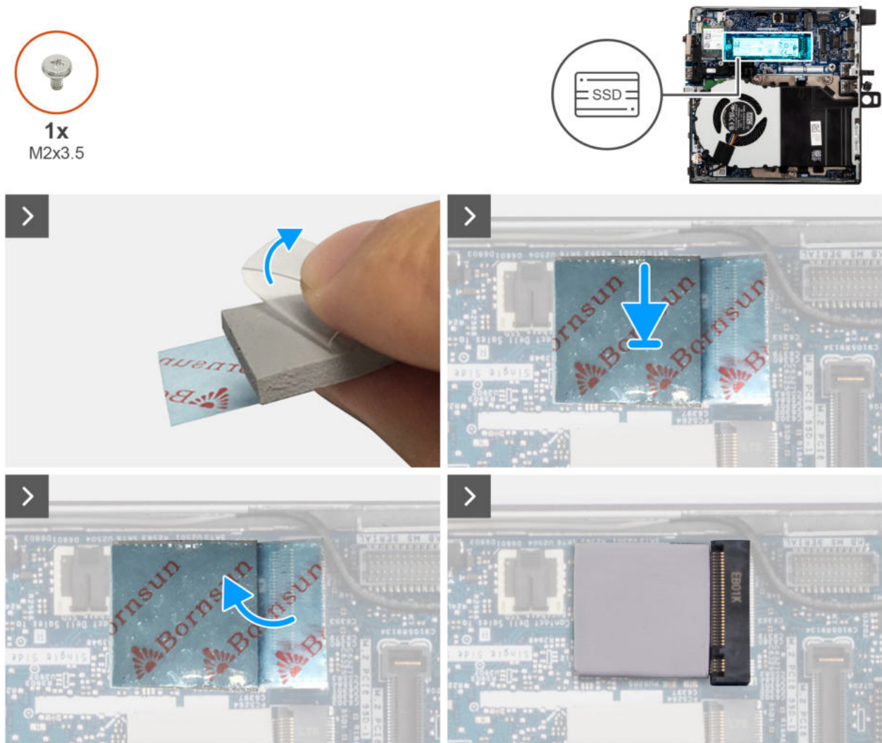
Figure 20. Installing the M.2 2280 solid-state drive
