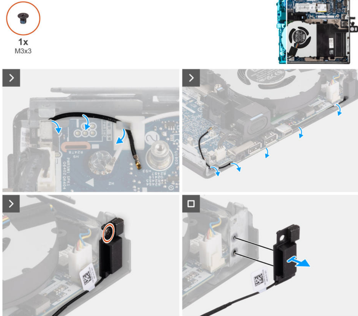
Figure 70. Removing the antenna module (black cable)
