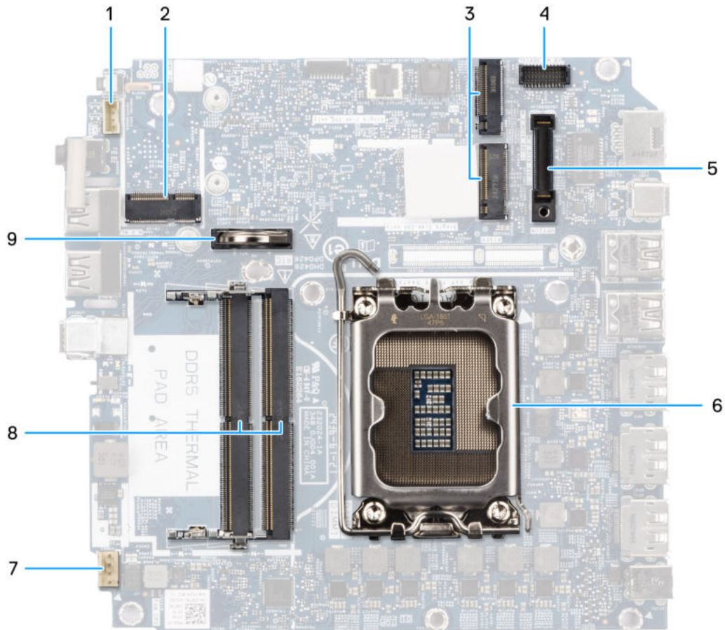
Figure 83. System board connectors
