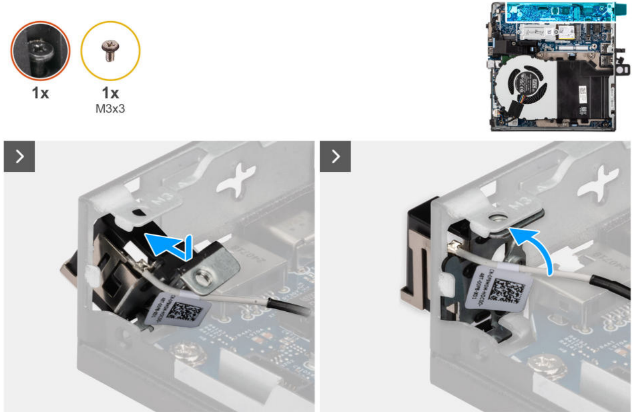
Figure 74. Installing the antenna module (white cable)
