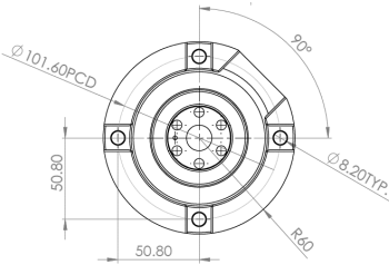
Jaegar PT Platform Mounting Pedestal
