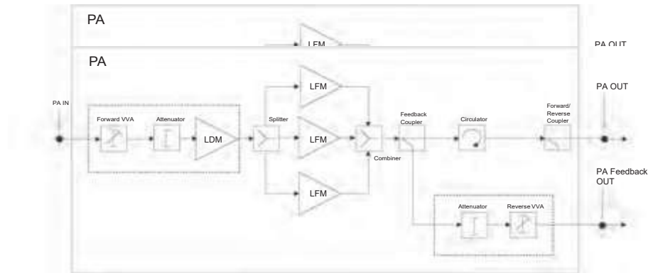
Figure 181: High-power PA Functional Block Diagram
