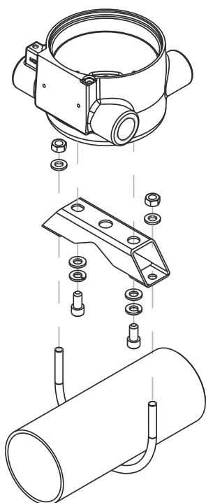
Figure 13: Optional Mounting
