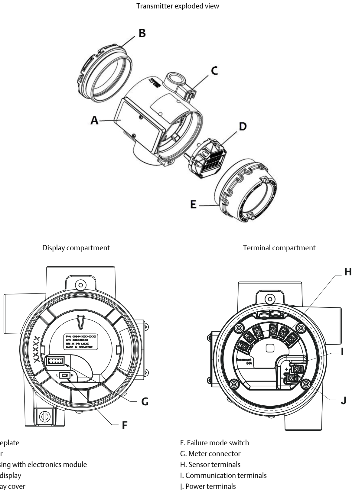
Figure 4: Rosemount 644 Field Mount
