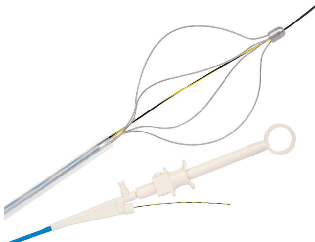
Lithotomy baskets, “Easy-Catch” with nozzle for contrast medium, for guide wire 0.035 inch , suitable for lithotripsy
