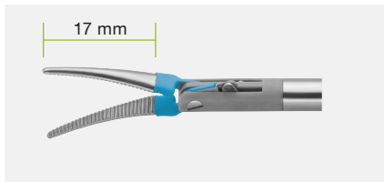
340 mm Ø 5 mm | LP450-001
