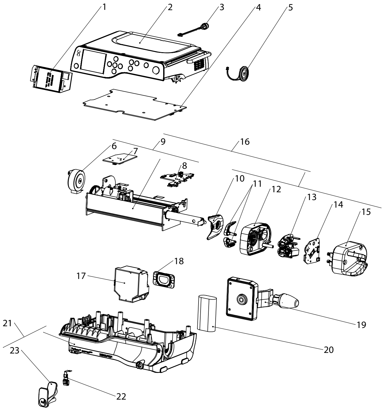
Fig. 8 - 1 Exploded drawing Perfusor® compact plus
