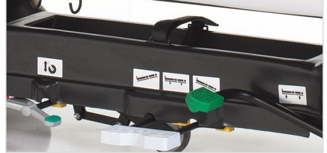
Oxygen tank holder integrated on sub-frame, 12Liter
