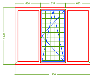
1. Ferestre; 1900-x1400(h)
