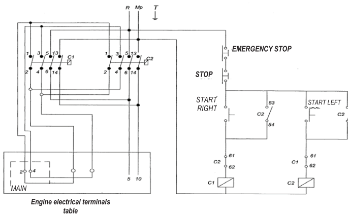
ELECTRICAL DIAGRAM FOR COOLED MEAT MINCING MACHINE
