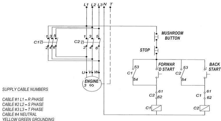
ELECTRICAL DIAGRAM FOR MONO PHASE MINCING MACHINES
