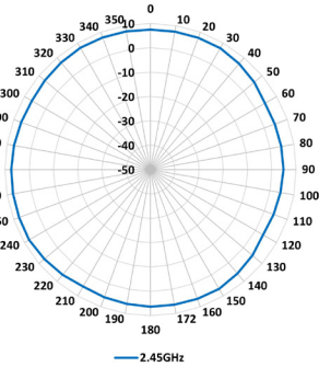
2.4GHz Band - Azimuth
