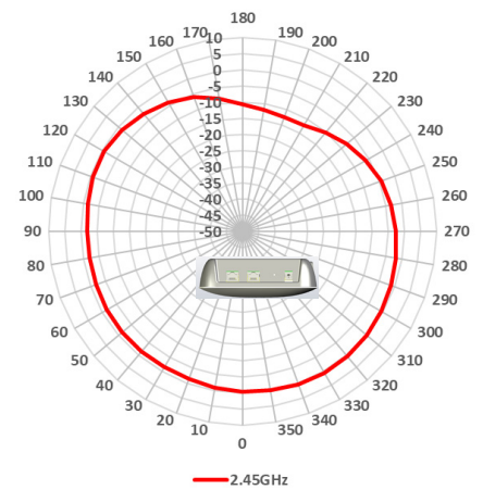
BLE/ZigBee Elevation
