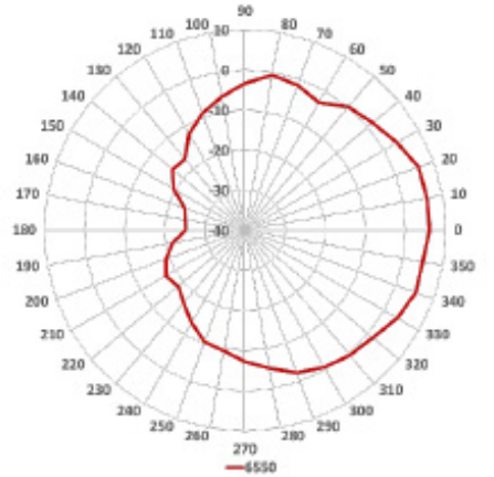
6.0GHz Elevation
