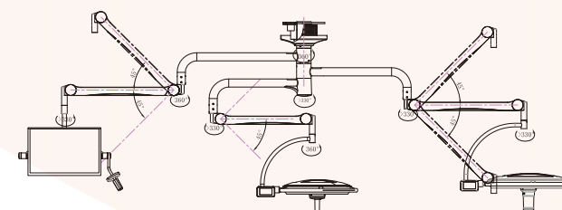
LUCKYSTAR E628/S628CD
