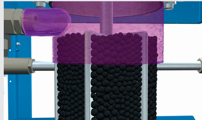
2. The pre-heated air flows into the integrated BOGE converter.
