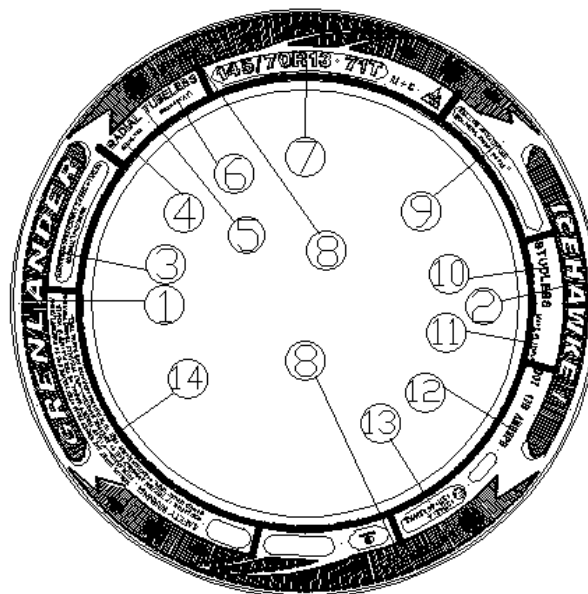
Lower mold
