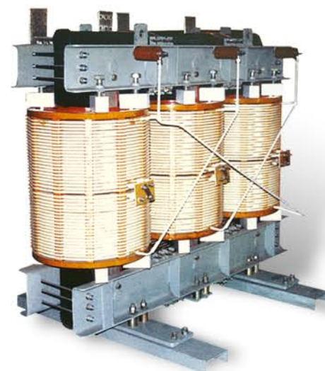
敞开通风干式变压器 Ventilated dry-type transformer
