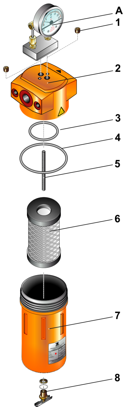
Exploded view
