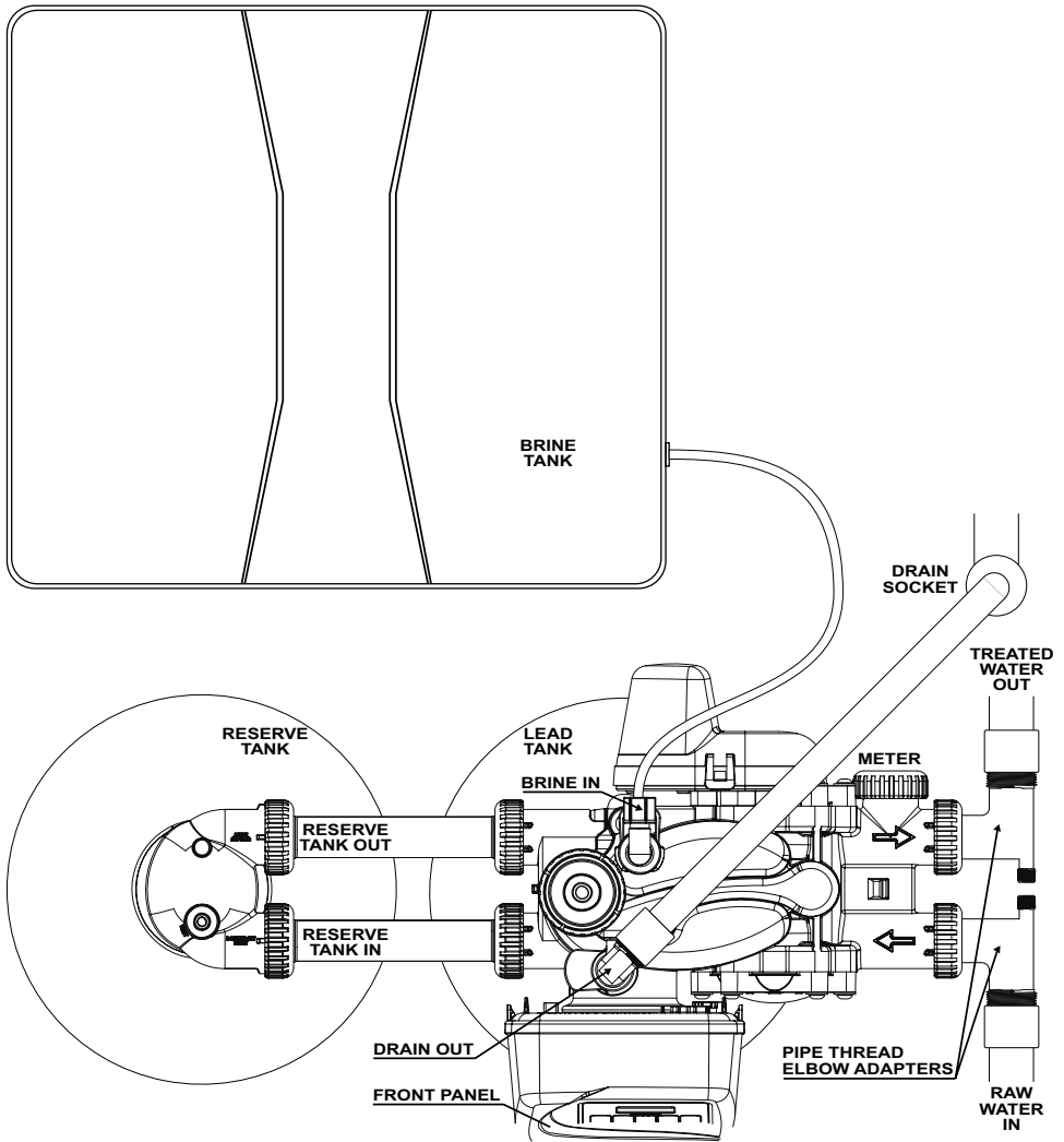
Ecosoft FU Twin/FK Twin piping connections top view
