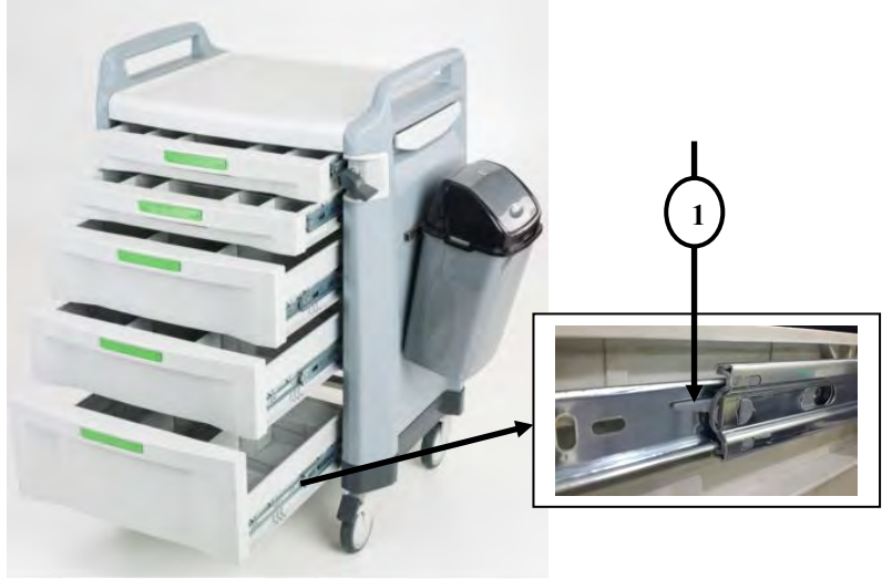
Figure 4. Removing the Drawers
