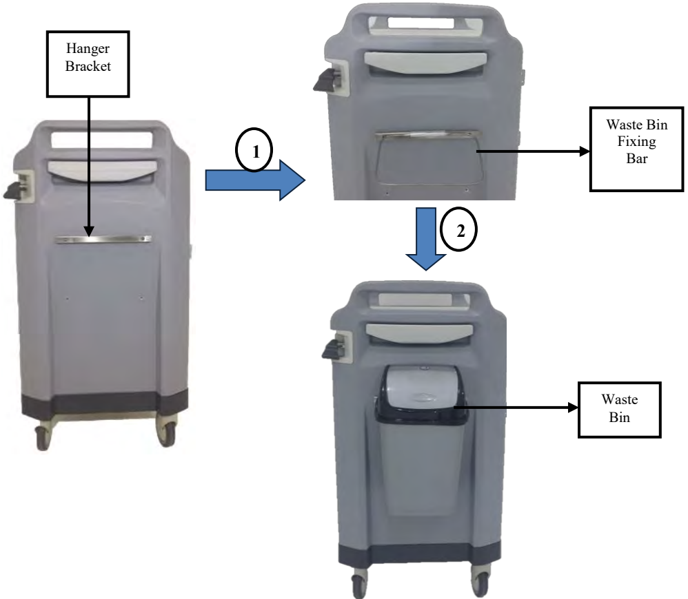
Figure 7. Waste Bin Installation
