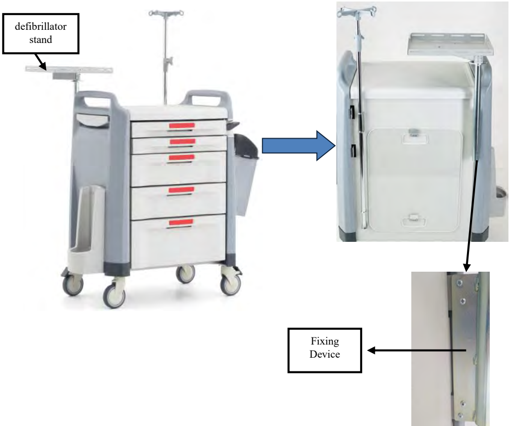
Figure 9. Defibrillator Stand Assembly
