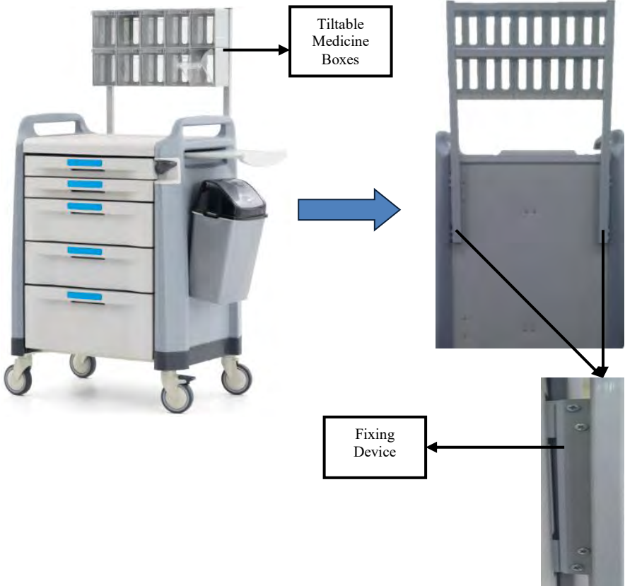
Figure 8. Installation of Tiltable Medicine Boxes
