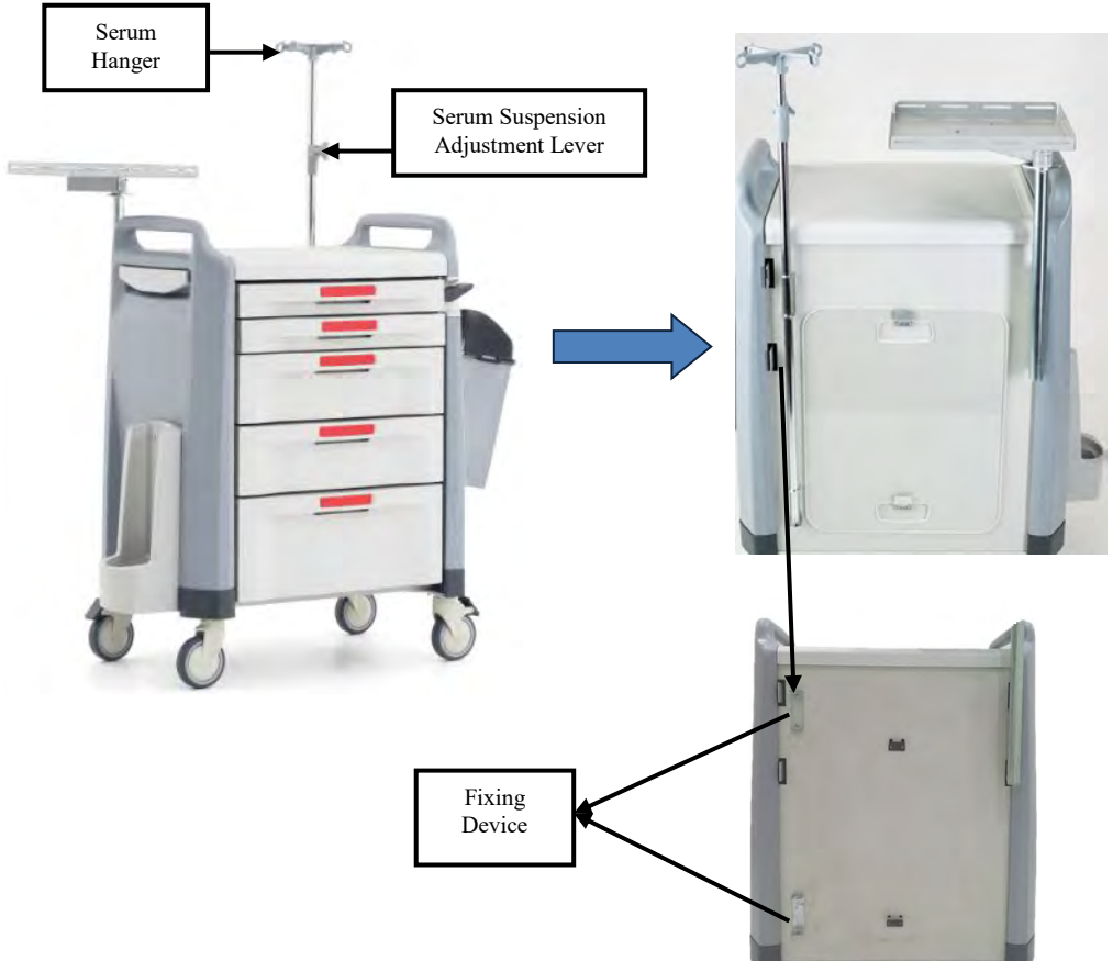
Figure 10. Assembling the IV Hanger
