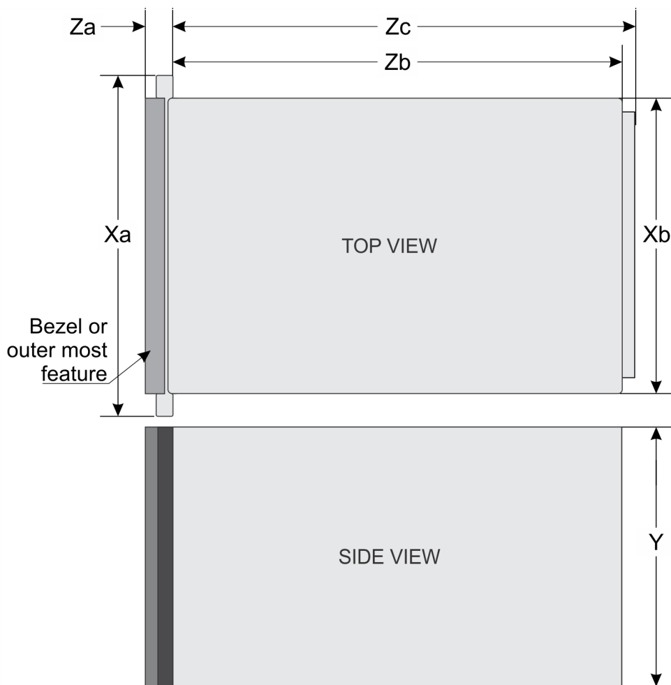
Figure 8. Dimensions of the PowerEdge MX7000
