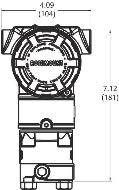
Figure 8: Rosemount 3051C Coplanar Flange
