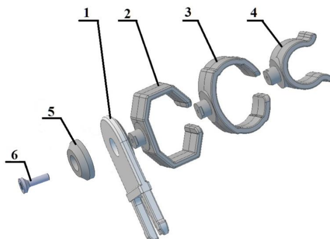
Fig. 11 Upper connector for attaching torches.
