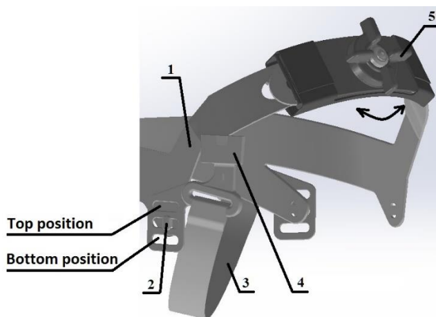
Fig.14 Band belt with suspension belt 1.Band belt; 2. Mounting hook; 3.Suspension belt; 4. Latch (1,2); 5.Knob
