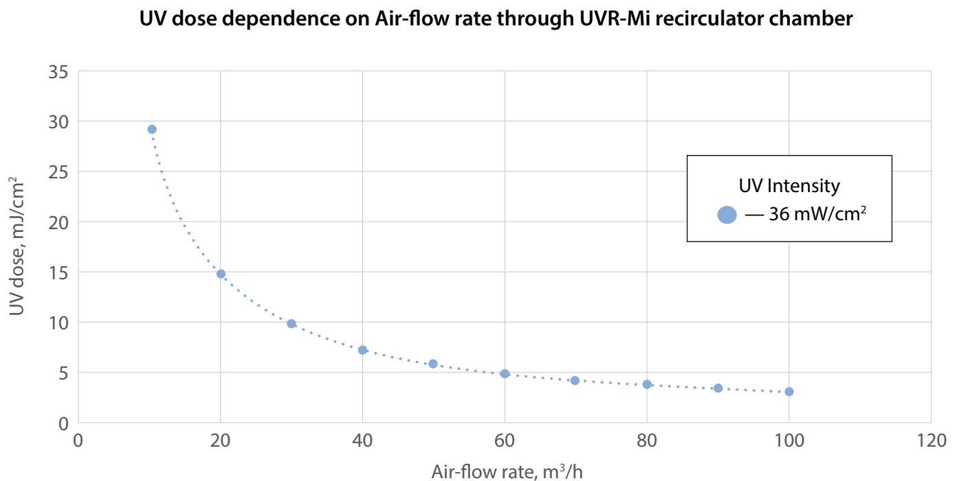
Figure 8: The relationship between the air-flow rate of UVR-Mi by Biosan and the UV dose received within it per one cycle.
