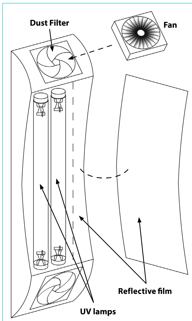
Figure 5: Construction schematics of a UV cleaner-recirculator UVR-Mi by Biosan. Forced by a fan, air passed through one filter into the chamber where it gets exposed to the UV emitted by the lamps then, decontaminated air leaves the chamber.
